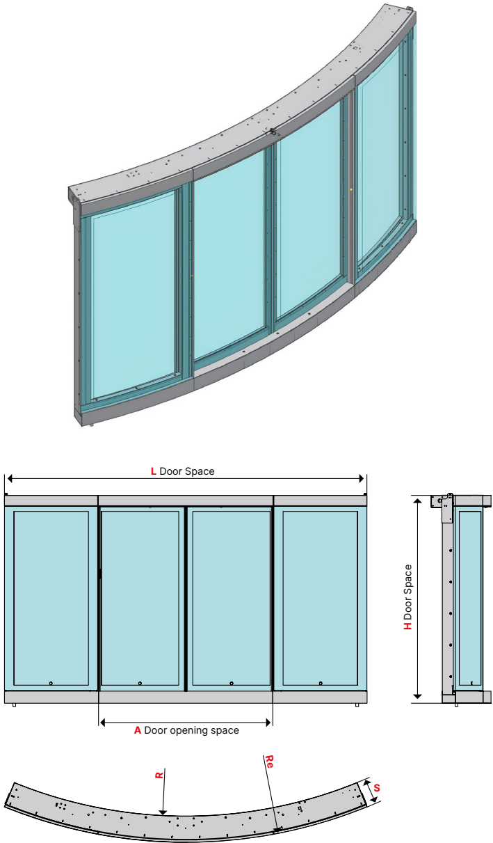
Doors with inflatable gasket
